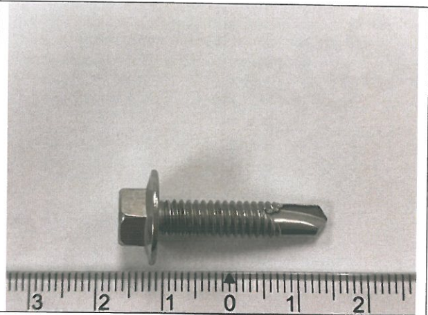
Appearance of NSSC 550 IND HEX WASHER HEAD DRILLING SCREW CSD(#12x1")-1 after 8000 hours salt spray test
