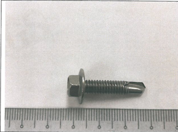
Appearance of NSSC 550 IND HEX WASHER HEAD DRILLING SCREW CSD(#12x1")-1 after 3000 hours salt spray test
