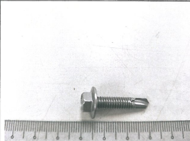
Appearance of NSSC 550 IND HEX WASHER HEAD DRILLING SCREW CSD(#12x1")-1 after 1000 hours salt spray test
