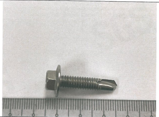
Appearance of NSSC 550 IND HEX WASHER HEAD DRILLING SCREW CSD(#12x1")-1 after 4000 hours salt spray test
